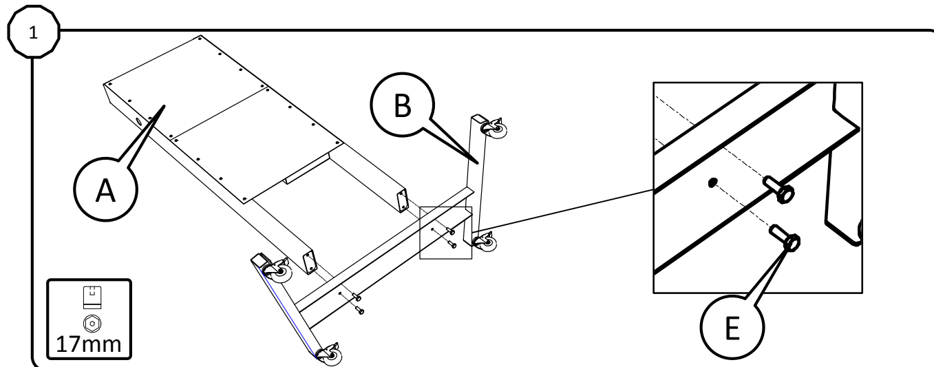
Assemble (● 17 mm)
