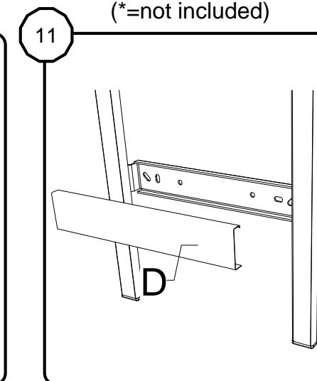
Mount cover
