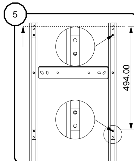
Measure and fix (● 4 mm)
