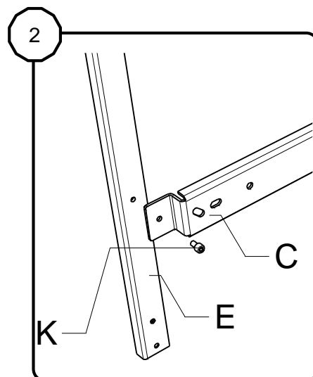
Assemble (● 5 mm)
