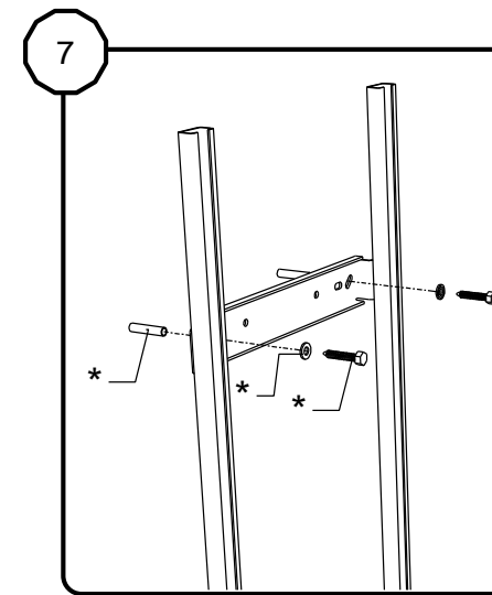
Fix to the wall 3x, fasteners not included
