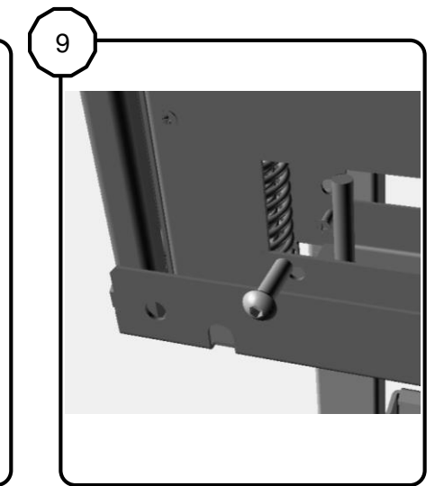
Hang LiftBox (*) and fix at bottom, use screw J (● 5 mm) NOTE: careful not to damage grey plastic dampener!
